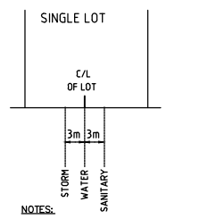
TYPICAL LOT SERVICING N.T.S.
