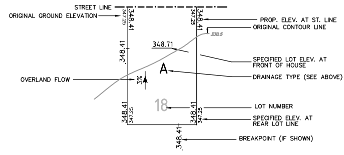
TYPICAL LOT GRADING N.T.S.
